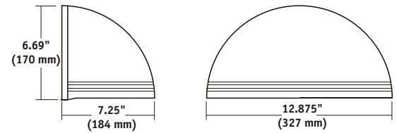
QSPC HID/CFL
